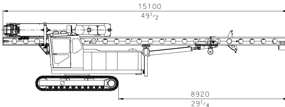
JUNTAN PM16 with HHK 3A hammer transport dimensions, leader equipped with hinge.
